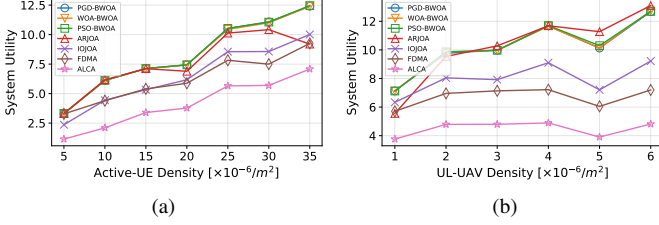
Fig. 3. (a) Utility versus active-UE density for WOA/PSO/PGD-BWOA (MF-SIC), force-all-offload, IOJOA, FDMA, and ALCA. (b) Utility versus UL UAV-server density.
