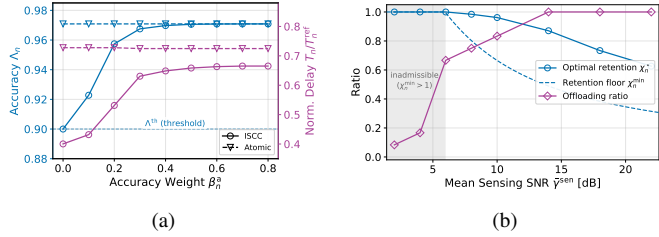
Fig. 4. ISCC effects: (a) accuracy-delay frontier swept over \beta^a , versus the atomic-task baseline; (b) optimal retention \chi_n^* , retention floor \chi_n^{min} , and ratio of offloading UEs versus mean sensing SNR.
