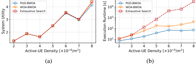
Fig. 2. Proposed BWOA matching inner PGD and WOA against exhaustive search, K = 3 : (a) attained utility, (b) runtime, versus active-UE density.
