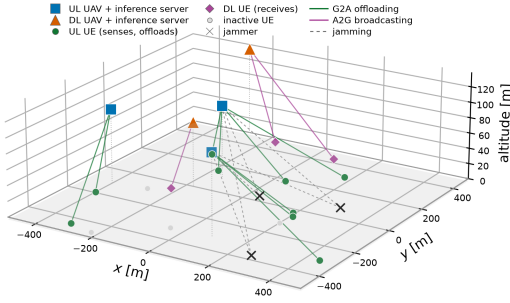
Fig. 1. One HPPP realisation of the SI-TNTN drawn by the simulator: UAVs hover at their sampled altitudes over ground UEs and jammers, with G2A offloading, A2G broadcasting, and jamming on both directions.
