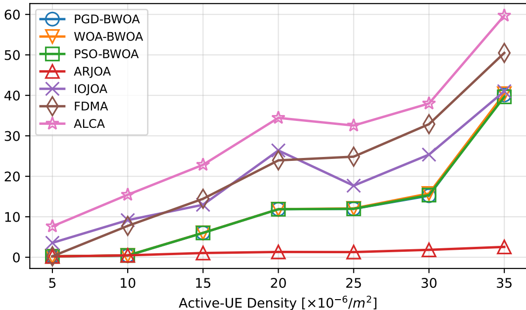
Total Energy Consumption [J]
