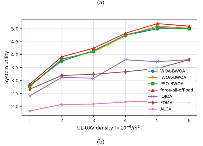
Fig. 3. (a) Utility versus active-UE density for WOA/IWOA/PSO-BWOA (MF-SIC), force-all-offload, IOJOA, FDMA, and ALCA. (b) Utility versus UL UAV-server density.
