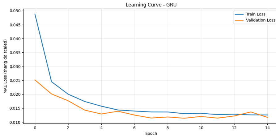
Hình 10: Learning curve — GRU (window=24h, hidden=64)
