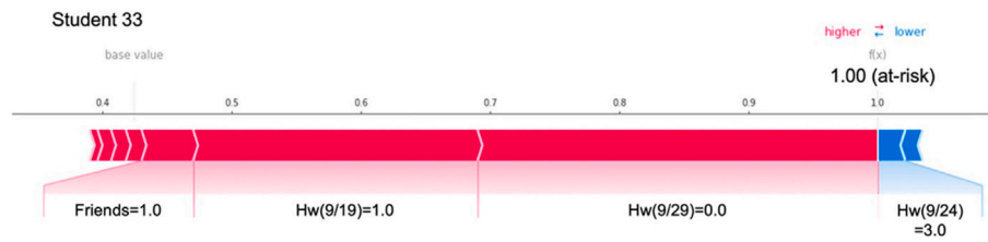
Fig. 12. Local SHAP explanation showing feature contributions for an at-risk student (Jang et al., 2022).
