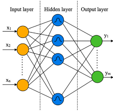
Fig. 5. Radial basis function network architecture.
