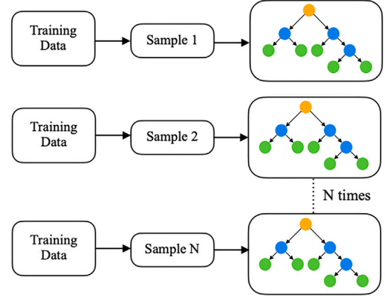
Fig. 2. Random forest algorithm workflow.
