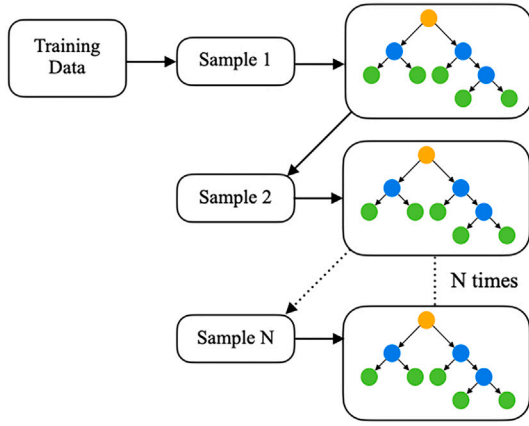
Fig. 3. Gradient boosting machine algorithm workflow.
