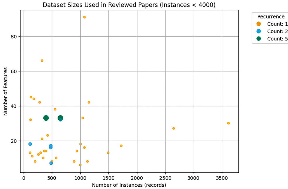
Fig. 9. Datasets sizes and recurrences (Instances < 4000).
