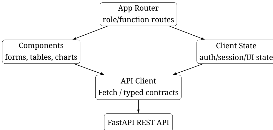
Hình 3.37: Web Application Architecture.
