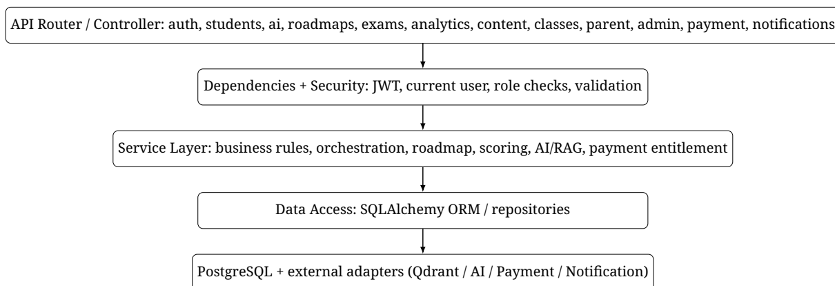
Hình 3.36: Backend layered architecture.
