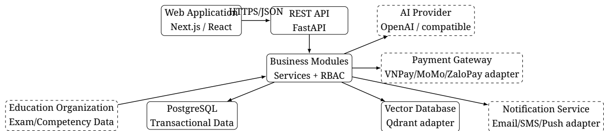
Hình 3.35: Overall System Architecture – AI-Edu Pathways.
