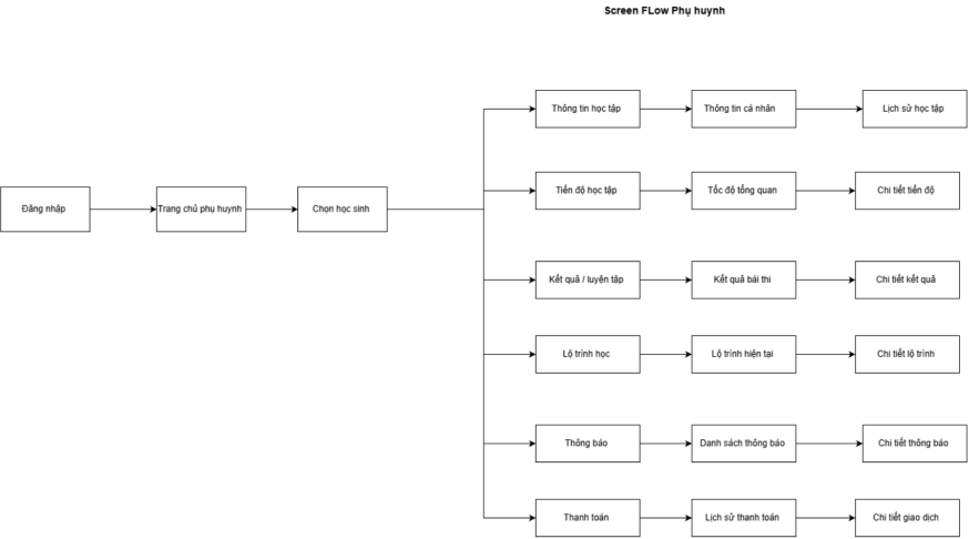
Screen Flow Phụ huynh
