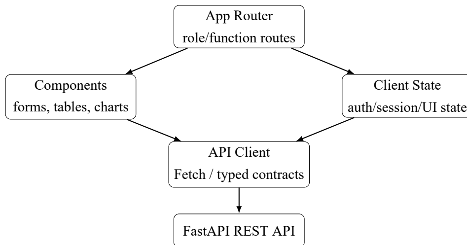
Hình 3.37: Web Application Architecture.
