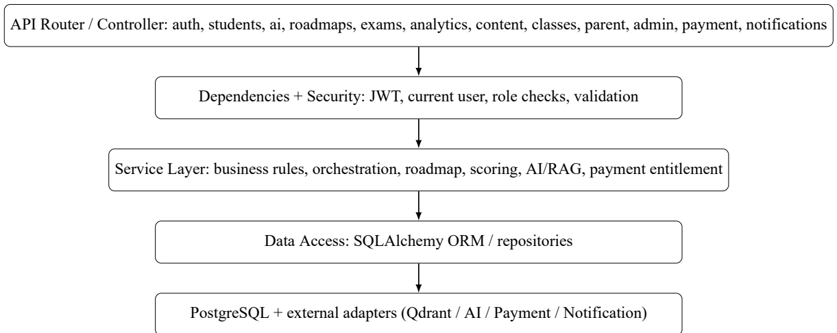
Hình 3.36: Backend layered architecture.
