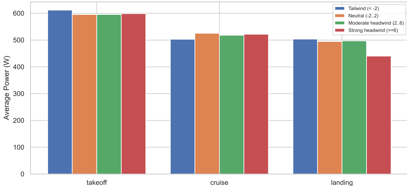
Average Power by regime and headwind condition
