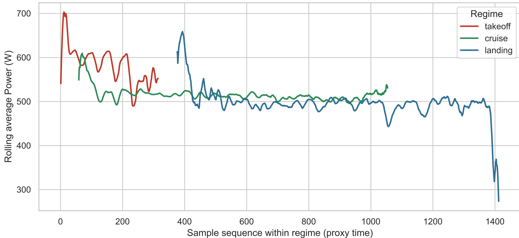
Power trend along flight progression, by regime
