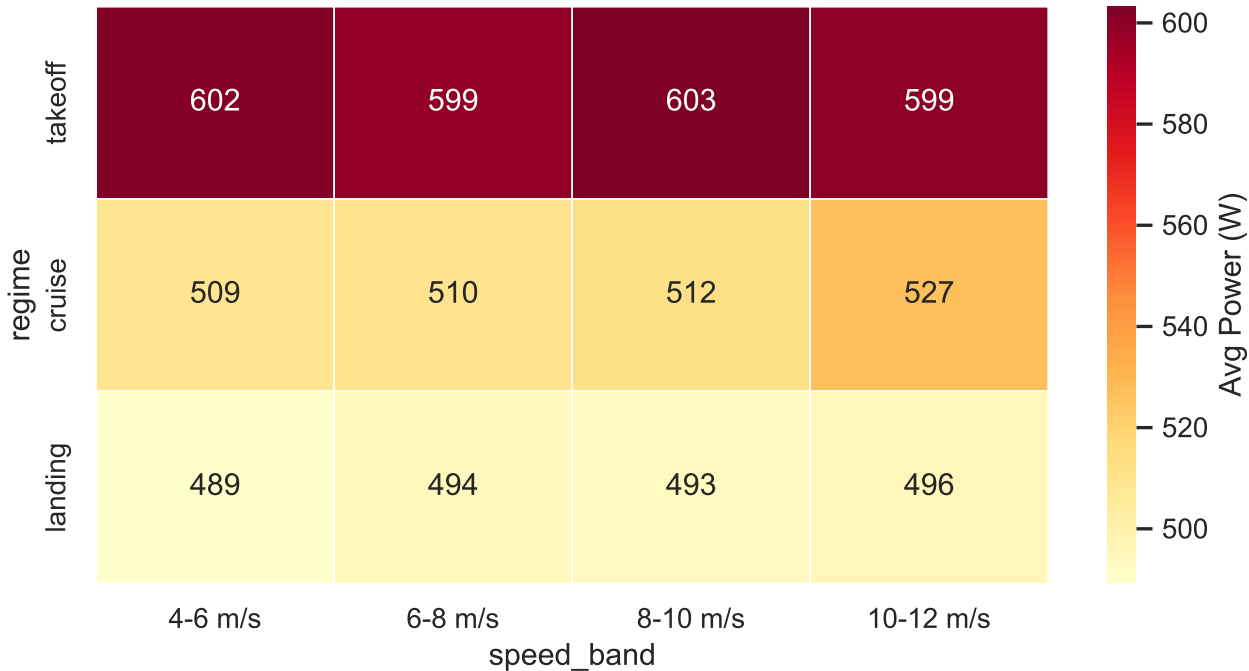
Average Power (W) — Regime × Speed band
