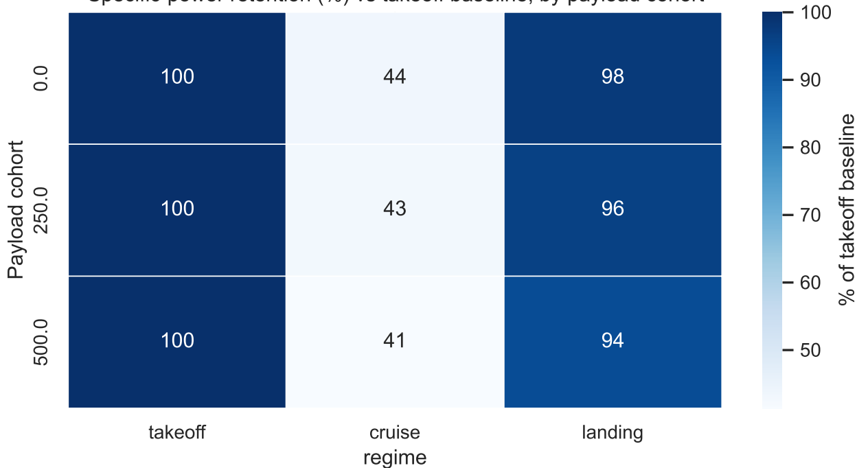
Specific-power retention (%) vs takeoff baseline, by payload cohort
