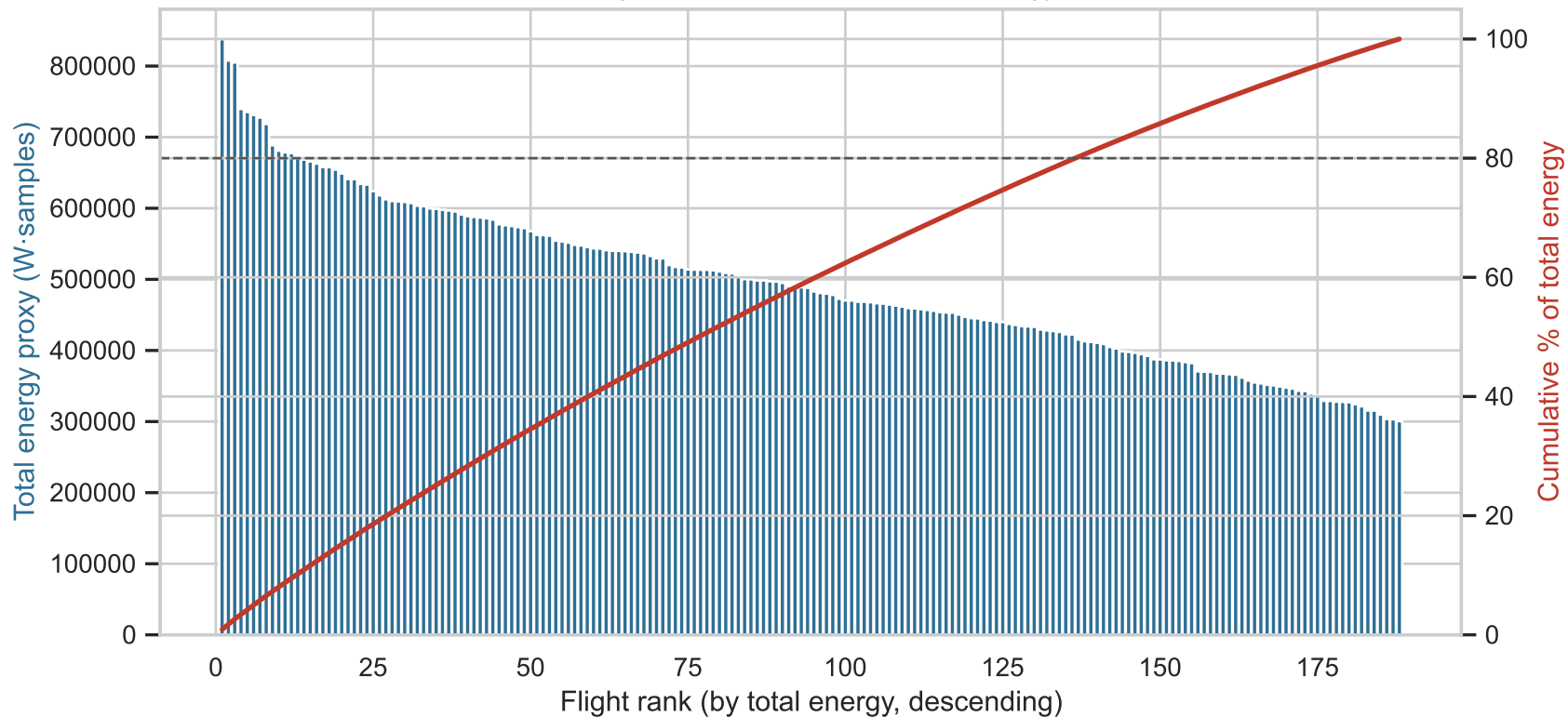
Pareto chart — flight contribution to total fleet energy consumption
