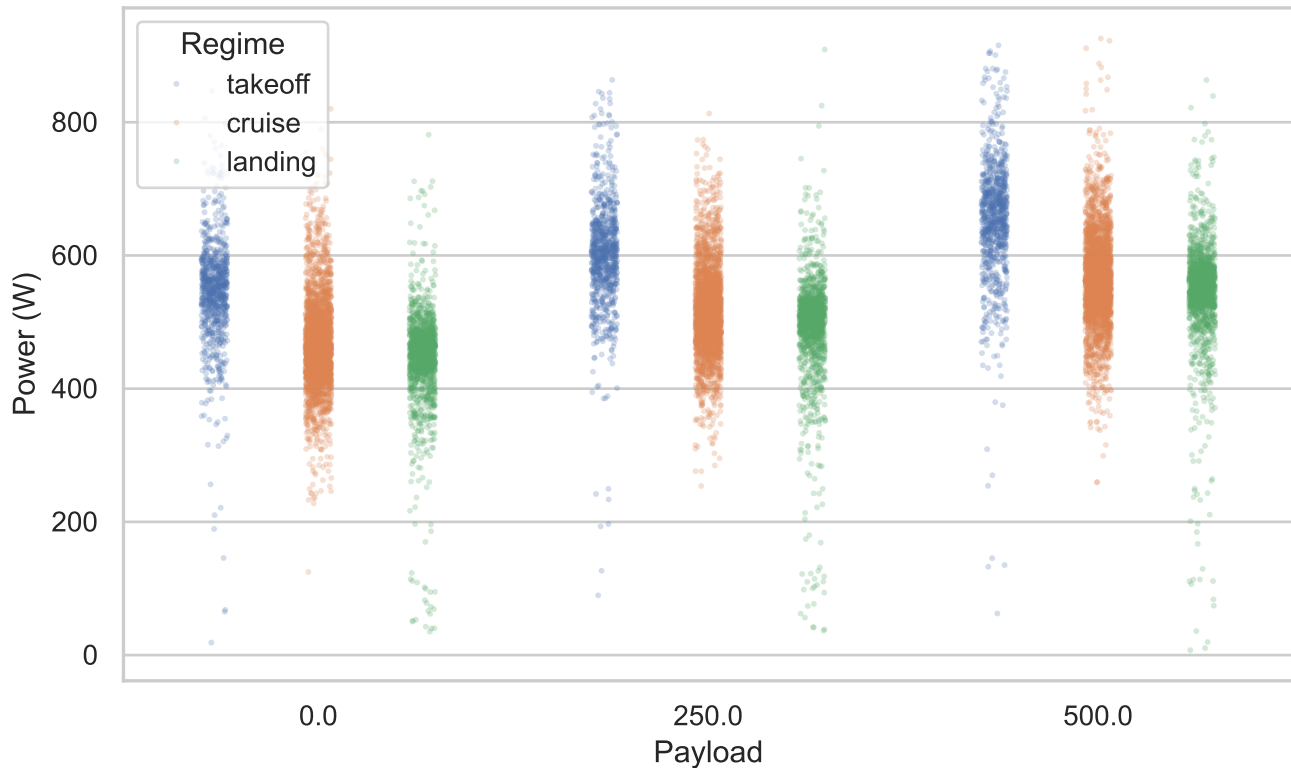
Power by payload level, split by regime (15k sample)
