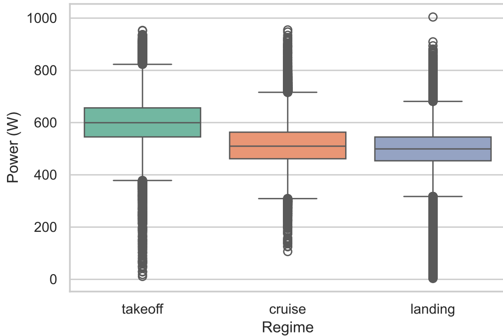
Power distribution by flight regime
