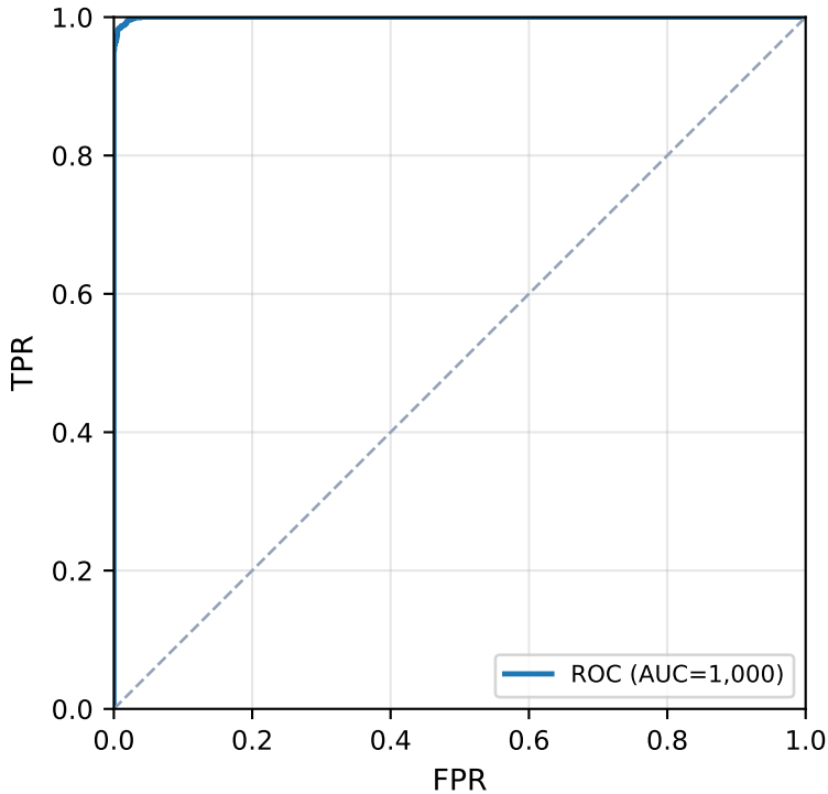
ROC — Conformer
