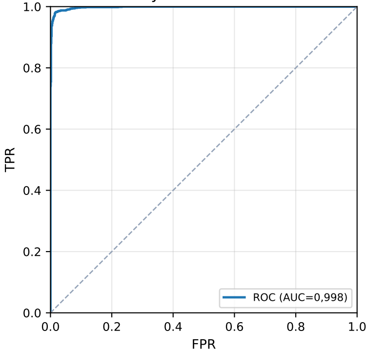
ROC — Hybrid CNN-Transformer
