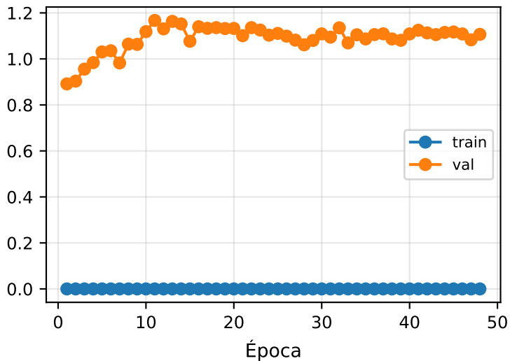
Loss
