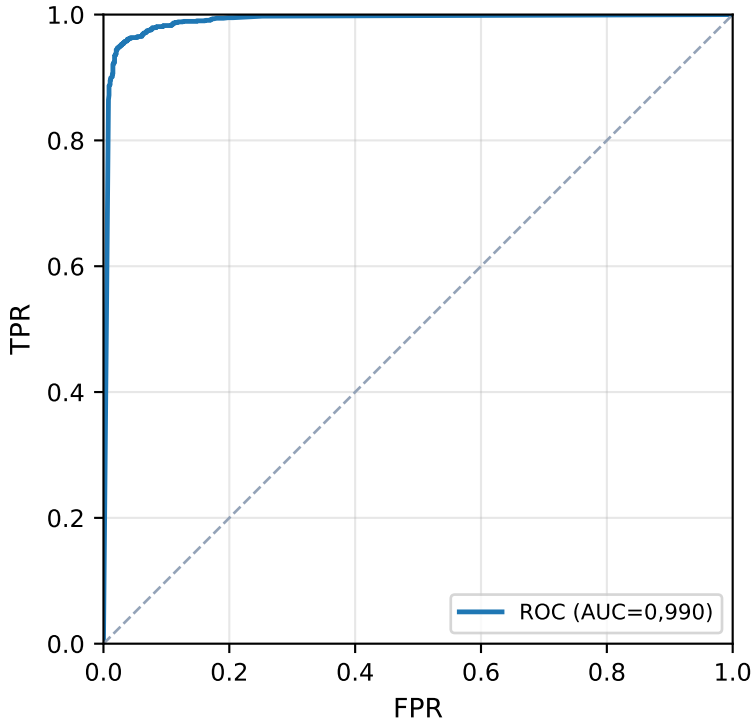
ROC — RawNet2
