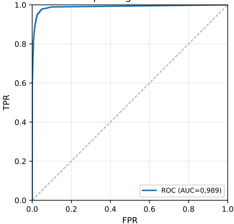
ROC — SpectrogramTransformer
