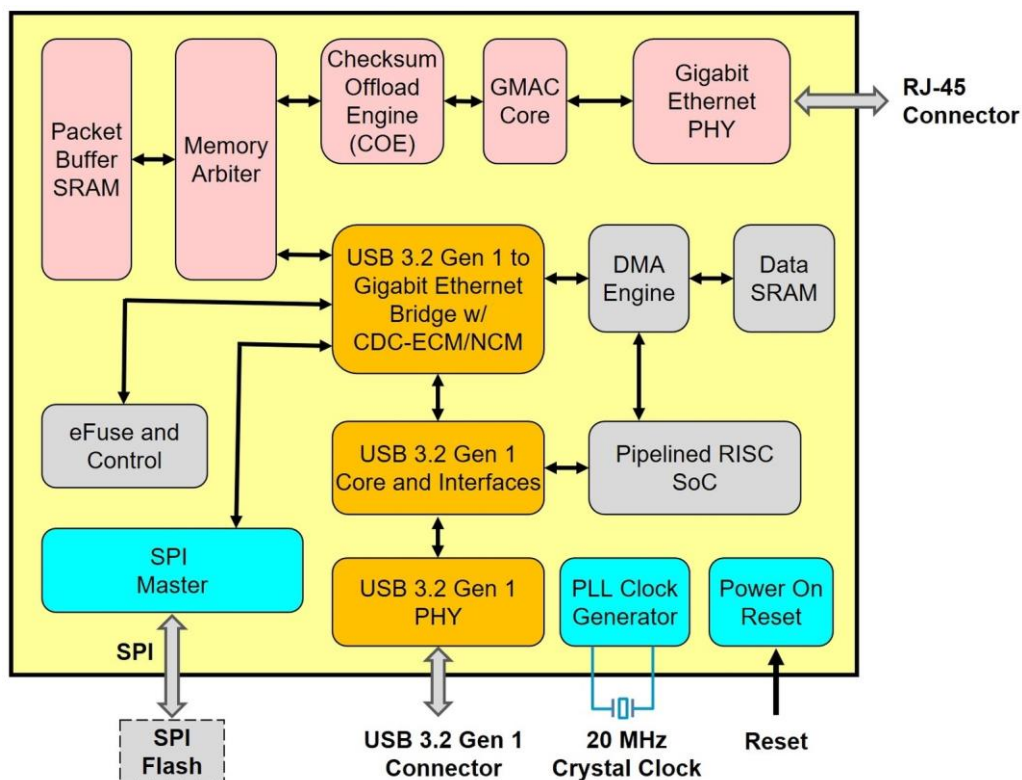
Figure 1. AX88179B Block Diagram
