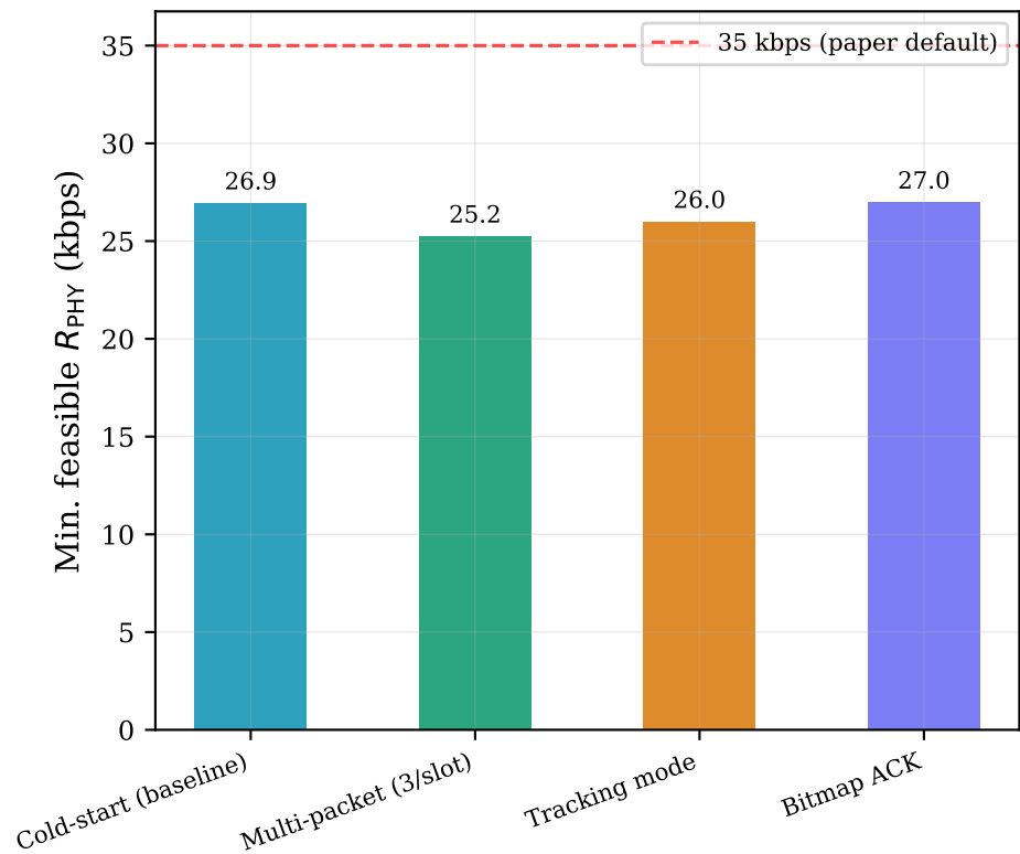
Minimum PHY Rate ( k_c = 100 , T_c = 10 s)
