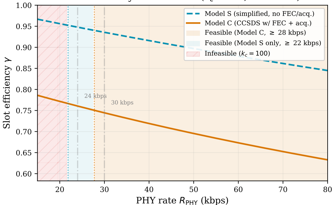
Slot efficiency vs. PHY rate ( k_c = 100 , S = 256 B)
