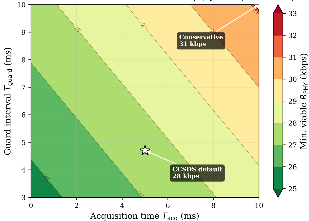
Minimum viable PHY rate for schedulability ( k_c = 100 , S = 256 B)
