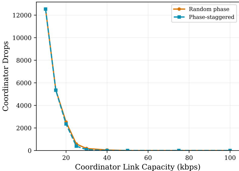
(a) Message Drops vs Capacity
