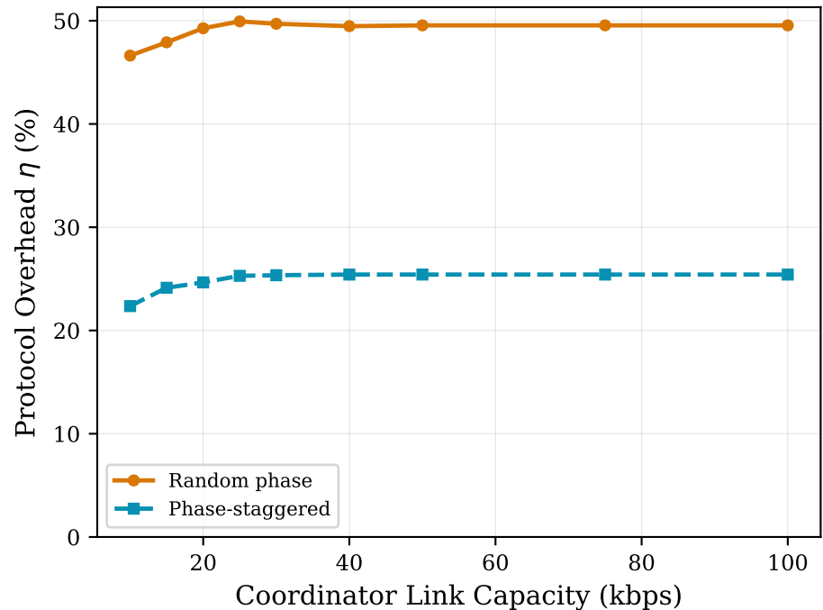
(b) Overhead vs Capacity
