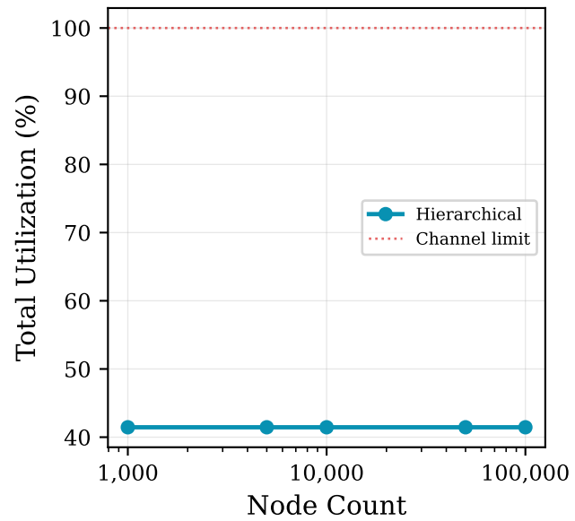
(c) Channel Utilization
