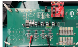
SiC high frequency inverter
