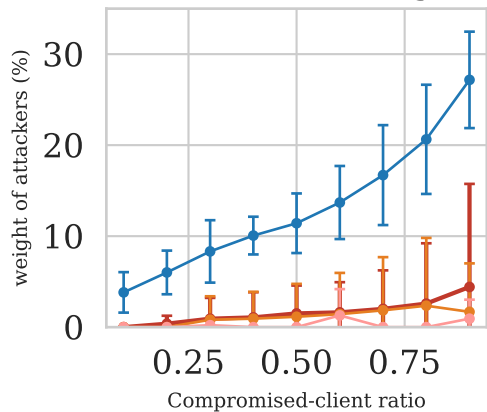
(c) Attacker weight
