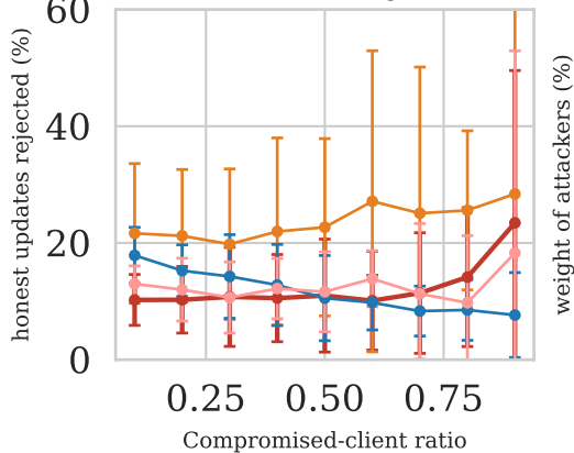
(b) Honest rejection
