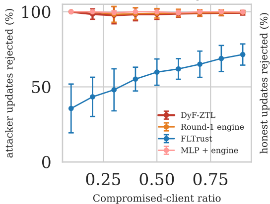
(a) Malicious rejection
