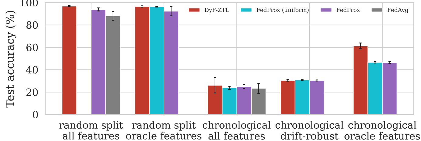
Random versus per-class chronological split and drift-aware feature sets
