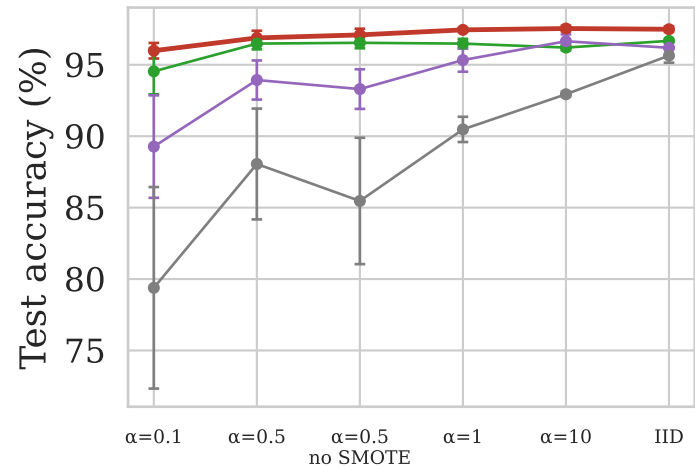
(a) Accuracy
