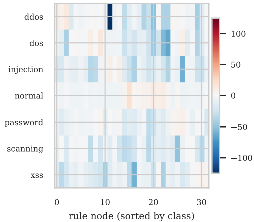
consequent weights
