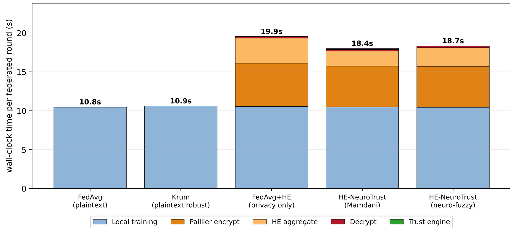
Per-round computational overhead breakdown (CIC-IoT-2023, 5 seeds). HE encryption dominates; the neuro-fuzzy trust engine is negligible.
