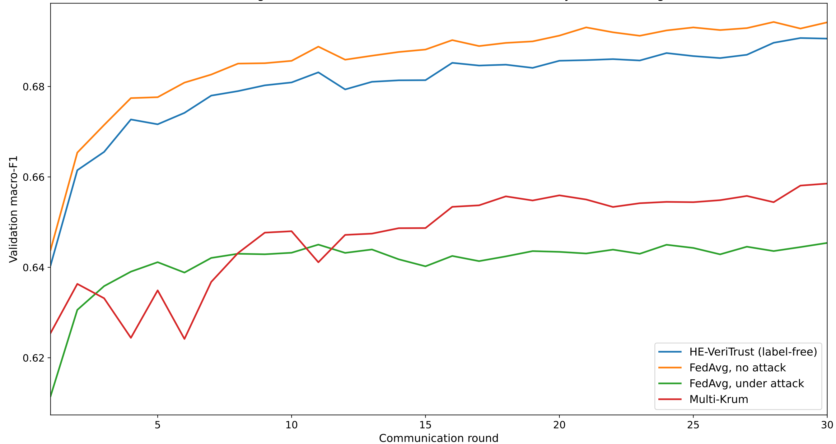
Convergence on CIC-IoT-2023 under the headline 30% Byzantine setting
