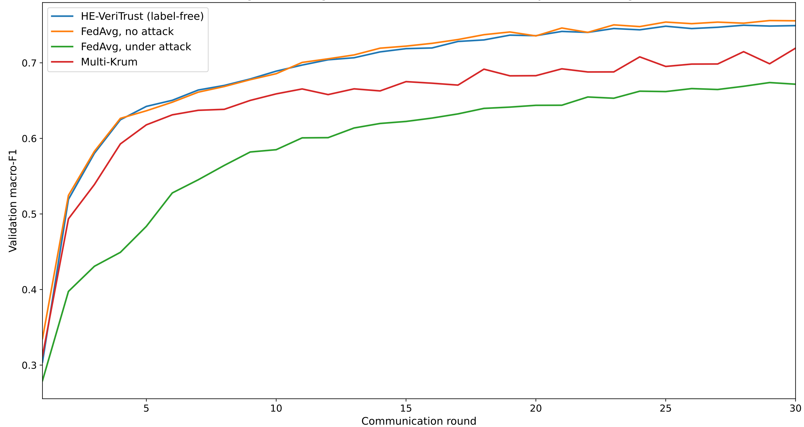
Convergence on Edge-IIoTset under the headline 30% Byzantine setting
