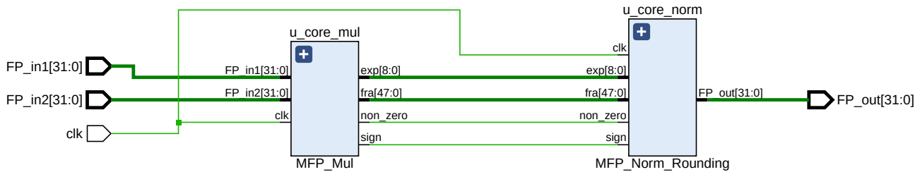
Figure 3.6: Block Diagram of the Multiplication Floating Point Unit
