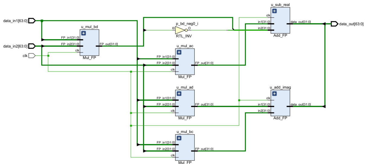
Figure 3.7: Block Diagram of the Complex Multiplier Unit
