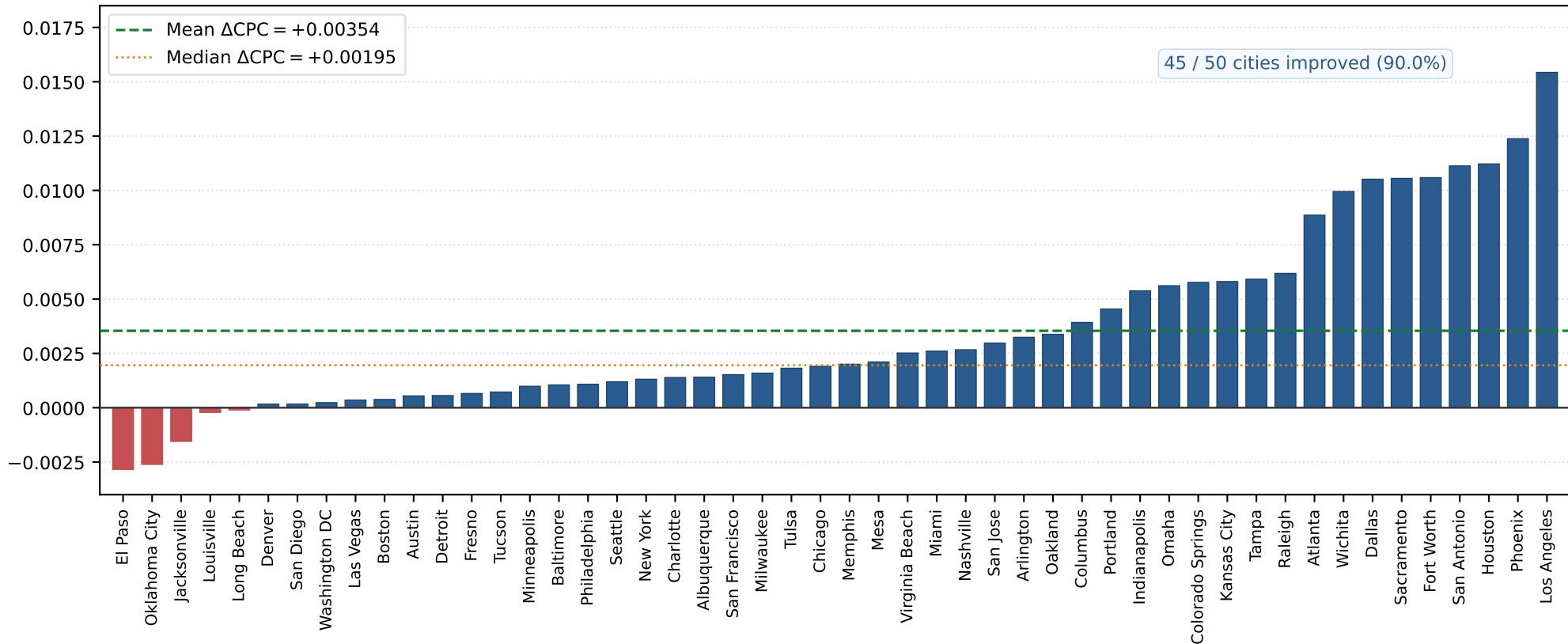
City-level improvement in interzonal CPC from oracle target-distance calibration
