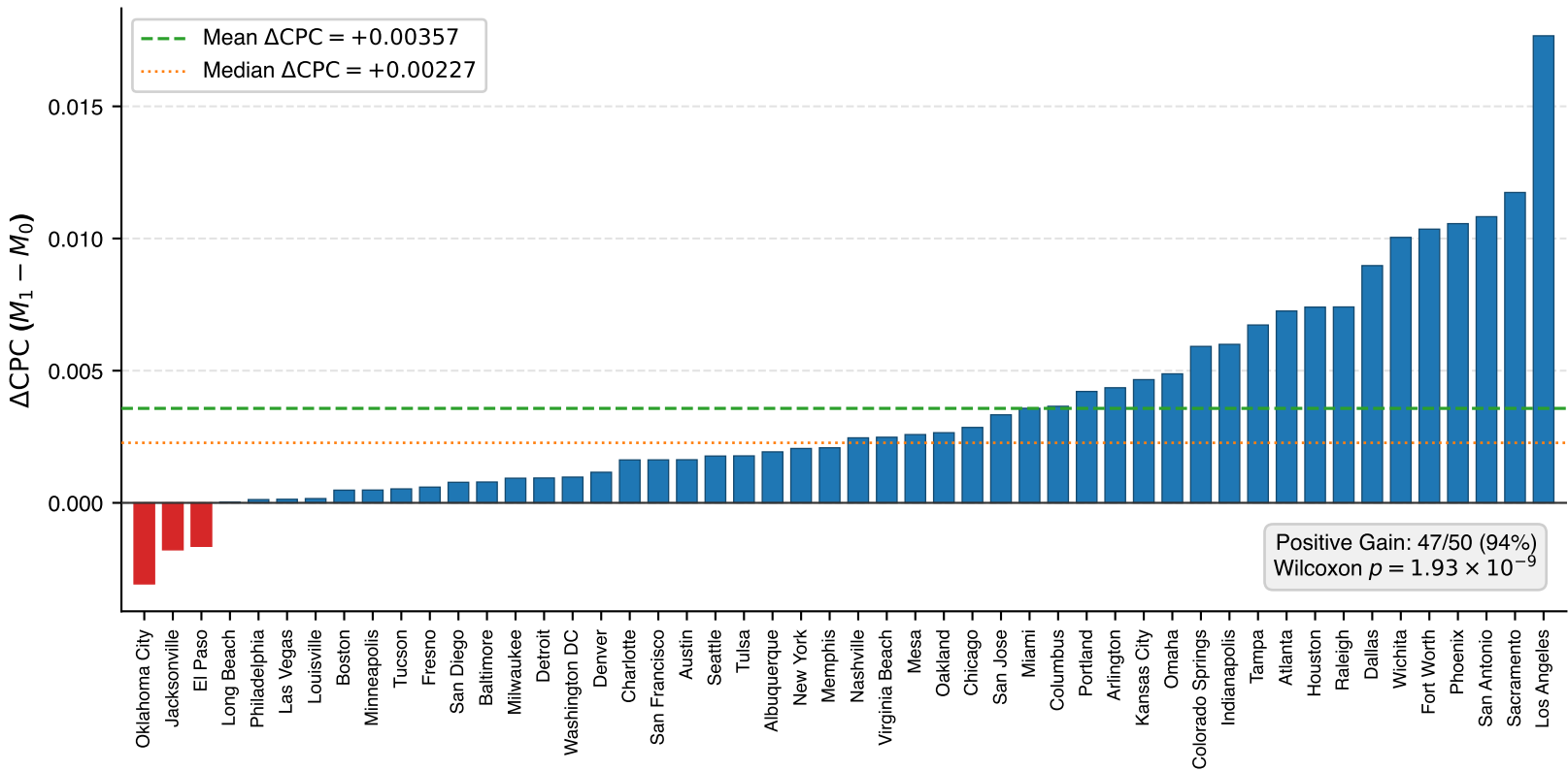
Zero-Shot OD Reconstruction Gain Across 50 U.S. Metropolitan Areas ( K = 8 )
