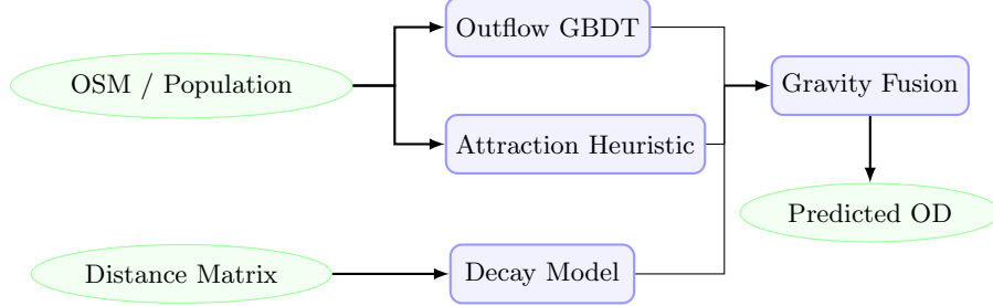
Fig. 3 Pipeline of the SDF-ZTF framework. Globally available spatial features are used to predict trip production ( O_i ) via a GBDT model and to compute destination attraction ( A_j ) via a training-free min-max heuristic. Distance decay is estimated separately from aggregate distributions. The components are combined via multiplicative gravity fusion to predict zero-shot flow matrices ( T_{ij} ).
