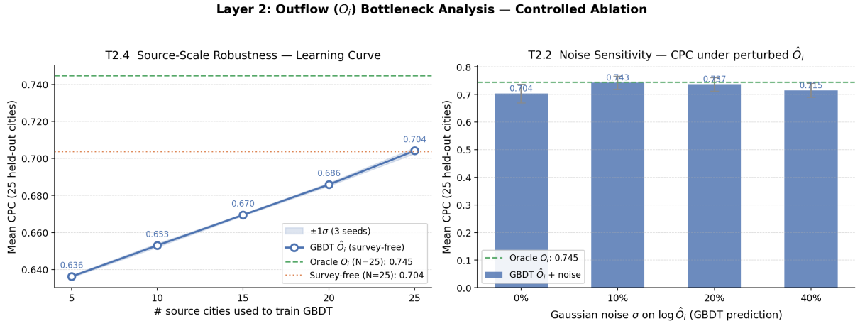
Fig. 9 Outflow Bottleneck Analysis (controlled ablation with fixed A_j heuristic and national decay prior). Left: Source-scale robustness learning curve — mean CPC \pm 1\sigma as the number of source cities used to train \text{GBDT}_{\hat{O}} increases from 5 to 25. CPC saturates by n_{\text{src}} \approx 15 –20. Right: Noise sensitivity — mean CPC \pm 1\sigma across 25 held-out cities under additive Gaussian noise \sigma \in \{0\%, 10\%, 20\%, 40\%\} injected on \log \hat{O}_i .
