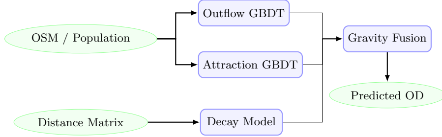
Fig. 3 Pipeline of the SDF-ZTF framework. Globally available spatial features serve as inputs to GBDT models predicting trip production ( O_i ) and attraction ( A_j ). Distance decay is estimated separately from aggregate distributions. The components are combined via multiplicative gravity fusion to predict zero-shot flow matrices ( T_{ij} ).
