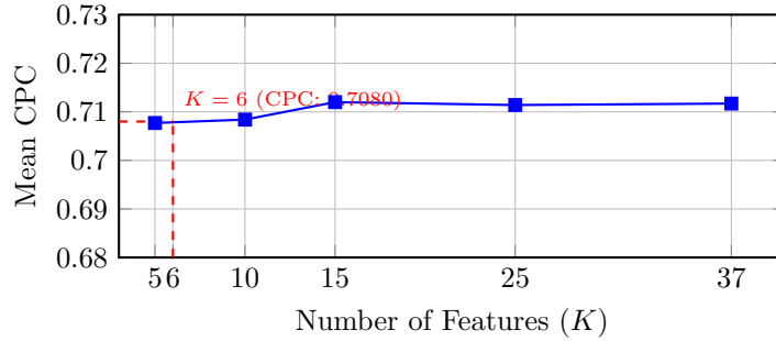
Fig. 7 SHAP feature count sweep over the 37-candidate feature set. While utilizing more than 6 features yields marginal accuracy gains, a parsimonious selection of 6 features is preferred to maintain generalization across diverse target-city environments.
