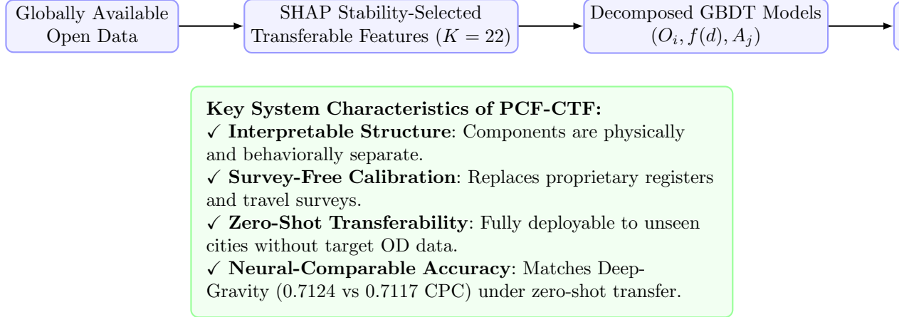
Fig. 11 Final takeaway diagram summarizing the zero-shot transferable pipeline (top) and key framework characteristics of PCF-CTF (bottom).
