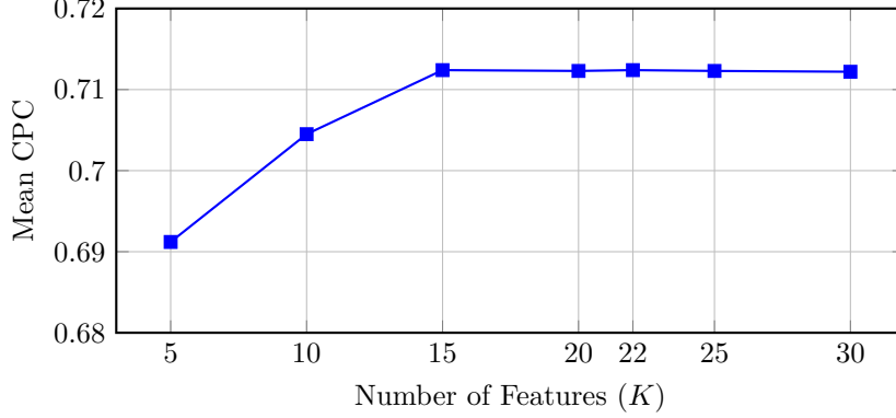
Fig. 9 SHAP feature count performance sweep showing zero-shot Mean CPC across the 25 held-out target cities. Performance peaks at K = 15 and plateaus through K = 22 and K = 30 features, validating our selection of exactly 22 stable features.
