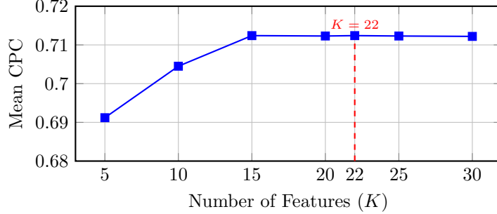
Fig. 7 SHAP feature count sweep: zero-shot CPC plateaus at 0.7124 from K = 15 onward, with K = 22 selected as it retains all features passing both stability thresholds ( \mu_p \geq 0.005 , S_p \geq 1.0 ), achieving 26.7% dimensionality reduction without performance loss.
