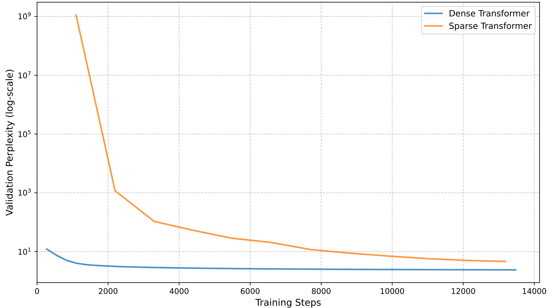
Dense vs. Sparse Transformer Perplexity Comparison
