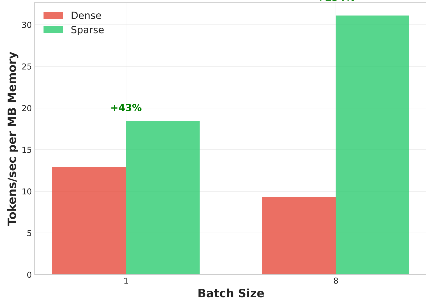
Memory Efficiency +234%
