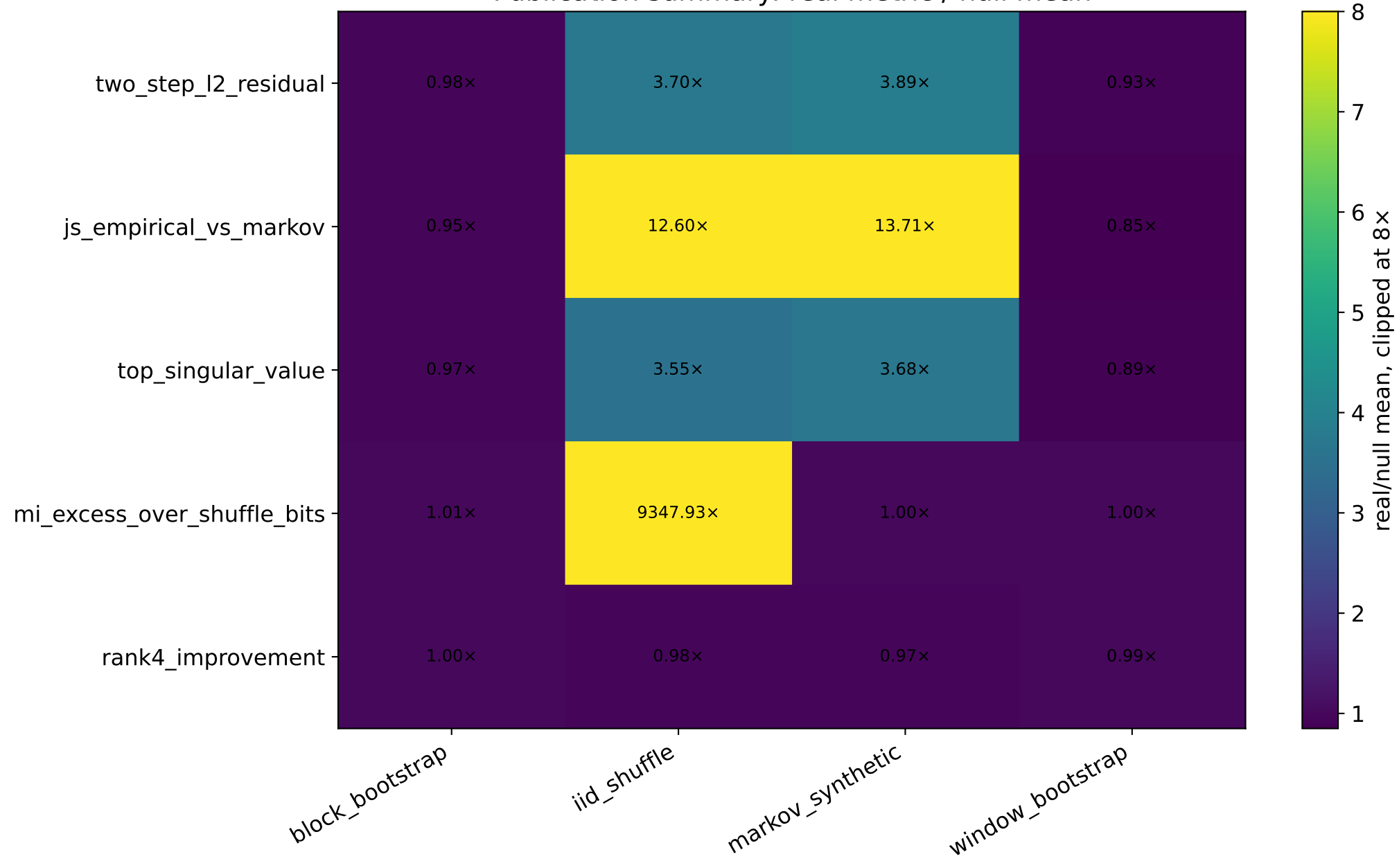
Publication summary: real metric / null mean
