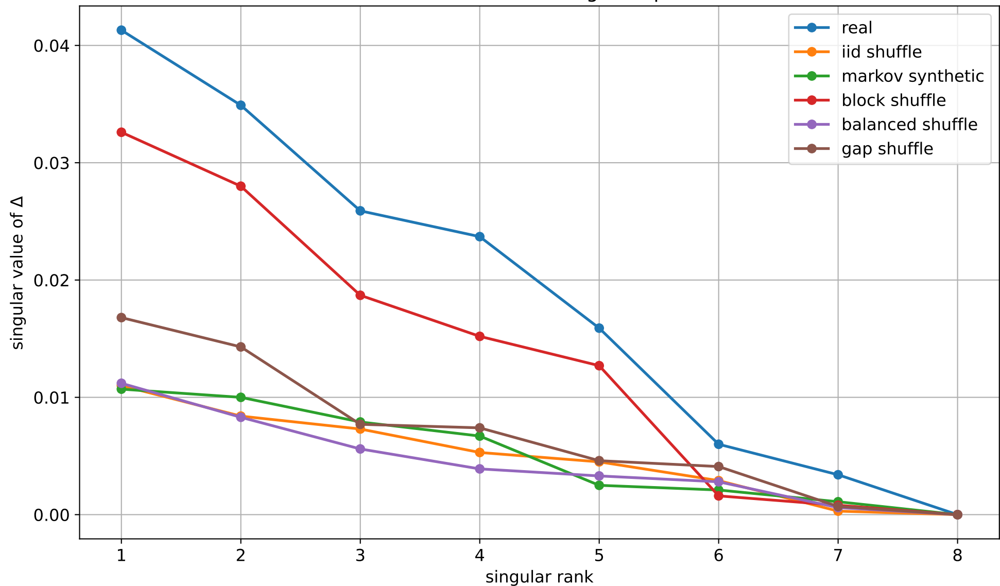
Real versus control singular spectra
