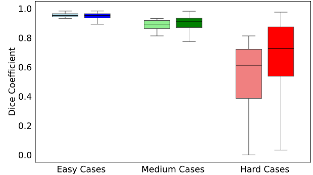
図 3 Performance Comparison by Difficulty Level on Kvasir-SEG dataset
