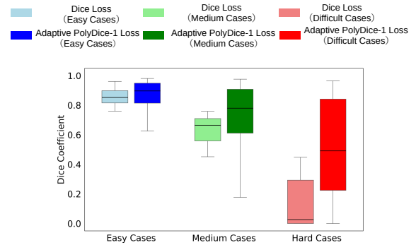
図 2 Performance Comparison by Difficulty Level on CVC-ClinicDB dataset
