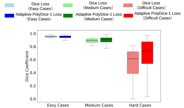
図 3 Performance Comparison by Difficulty Level on Kvasir-SEG dataset
