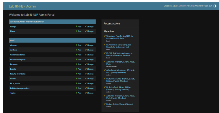
Gambar 3.8: Halaman Admin
