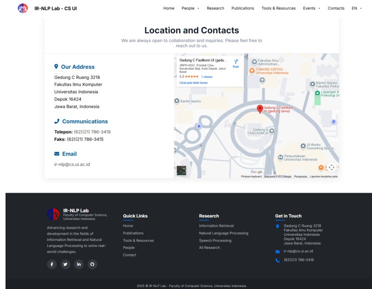
Gambar 3.7: Halaman Contact
